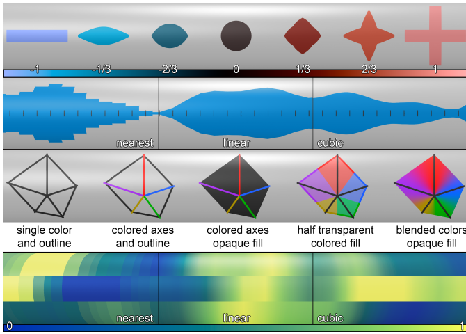
Fig. 3. Example configurations of the more complex glyph types and continuous mappings we implemented. 1st row: Sign glyph with diverging color (see color scale), showing the full value range from -1 to 1. 2nd row: Line plot with nearest, linear and cubic attribute interpolation. 3rd row: five configurations of a 5-axis Star glyph showing the colorization capabilities. 4th row: Temporal heat map , again with the three interpolation modes, showing values from 0 to 1. All interpolation takes place before mapping. Color maps used in 1st and 4th from [6] (berlin, imola).
