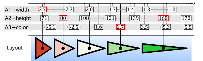
Fig. 8. Glyph placement at original samples: the first sample among mapped attributes A1, A2 and A3 that corresponds to a point on the trajectory where the glyph would fit decides the location of the glyph. The remaining attributes are interpolated (indicated by the grey arrows) before computing the value for the visual attribute.
