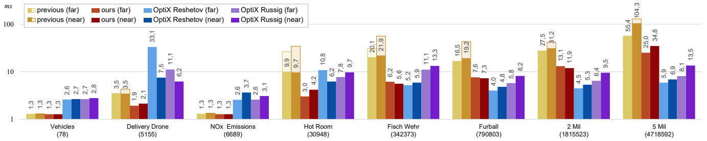
Fig. 11. Average render times (in milliseconds) of the eight evaluated data sets for far and near views using a logarithmic scale. Segment counts are given in parentheses. Numbers for previous state times with early-z culling enabled, while the transparent area depicts frame times without.
