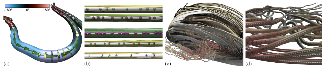
Fig. 1. Examples of multivariate on-tube visualizations. (a) Vehicles: steering angle is mapped to color (cf. color scale); Triangles show velocity mapped to length and acceleration mapped to color and inversely to base width (wide and purple depict braking actions); thin yellow Rectangles are used to show the throttle amount. (b) Delivery Drones: using color to visualize velocity (yellow = faster); Line plot shows power usage; Circles used as labels to identify drones. (c,d) Fisch Wehr: overview and detail visualizations of streamlines. Color shows velocity (red = faster); a Line plot is used to visualize high pressure areas; Sign glyph shows angular velocity (shape and color). Ambient occlusion emphasizes the vortex structure in (c).
