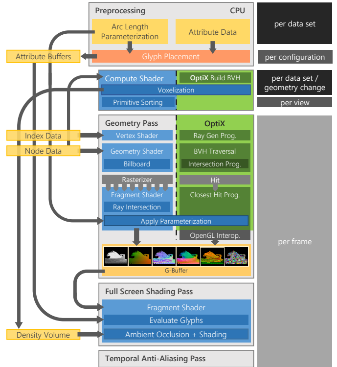
Fig. 4. Schematic illustration of the data flow and two-pass rendering process with its alternative render paths using either highly optimized rasterization or hardware-accelerated ray tracing.
