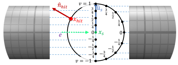
Fig. 6. Illustration of the two strategies to parameterize tube surface around center curve. Left: equidistant in screen space; right: arc length parameterization.
