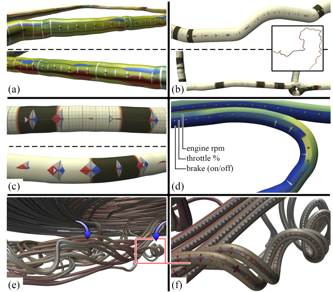
Fig. 10. Various examples of layer configurations supported by our tool. (a, b and c) are from NOx Emissions . (d) shows the Vehicles data set. (e and f) are views on the turbulent region of Fisch Wehr .
