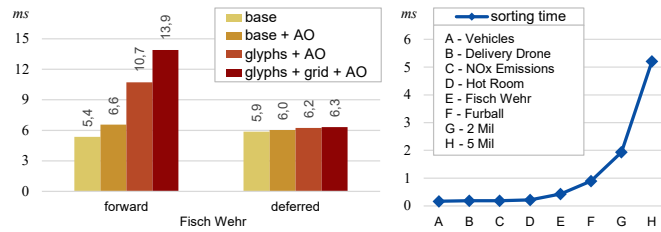
Fig. 12. Left: Comparing the influence of AO, glyph and grid mapping on the frame times for Fisch Wehr (averaged over both view configurations). A complex configuration of 4 glyph layers was used with a color- and normal-mapped grid. Right: Sort timings in milliseconds.
